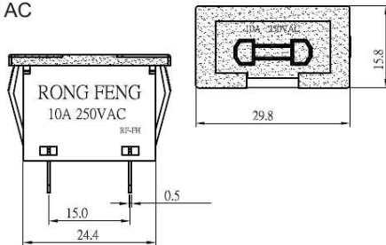
RF-FH(Fuse Holder)
